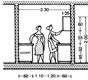
2 Section through kitchen; space for two people
